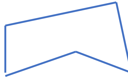
Concave Polygons
